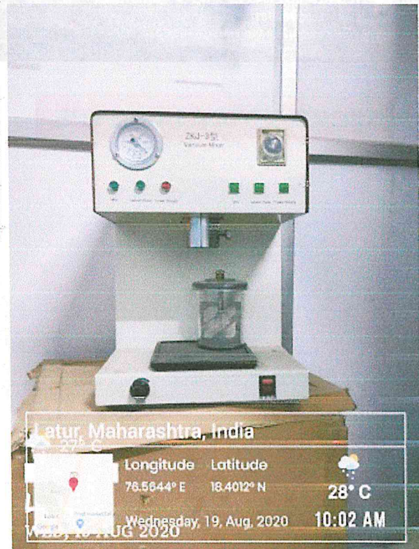
Vacuum mixing machine
