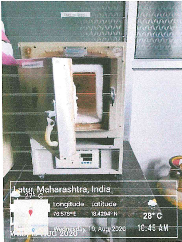
Burn-out furnace
